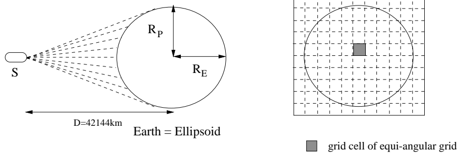
Figure 2: Geolocation parameters. Left = intersection of the lines of sight of a geostationary satellite with the Earth reference ellipsoid. Right = the corresponding equi-angular grid projection of the Earth as viewed from the satellite.
