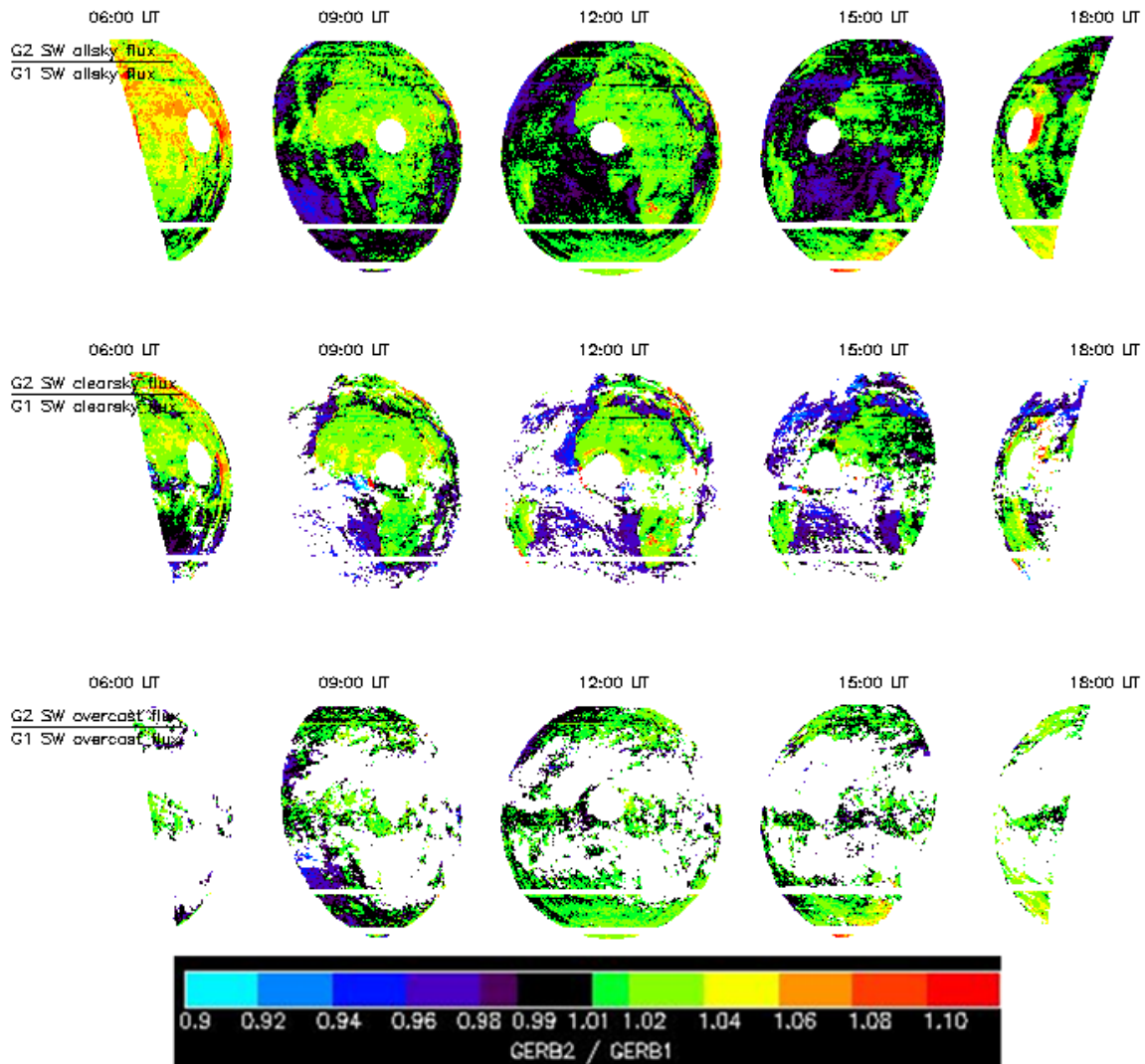
Figure 7. Shortwave G2/G1 average ratio plots for May 2007, for 5 times of day, decomposed according the GERB scene ID into allsky, clearsky and overcast.
