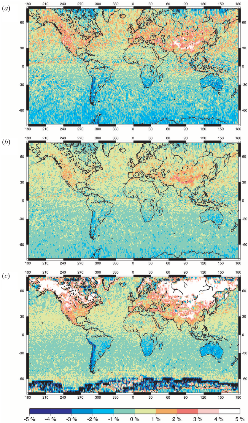
Figure 1. Annual average of the azimuth anisotropy \Delta (%) for the CERES: (a) infrared window channel, (b) broadband longwave channel and (c) infrared window channel under clear and partly cloudy conditions only.
