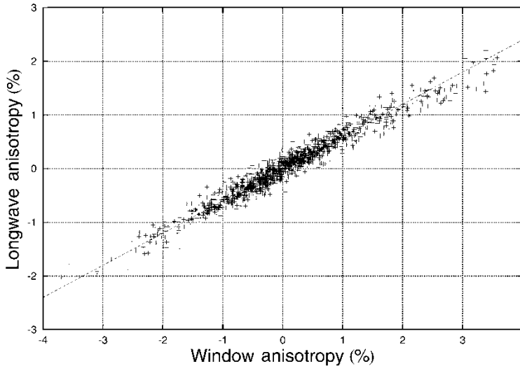
Figure 2. Scatter plot of the longwave versus the window anisotropies. Each dot corresponds to a 1^\circ \times 1^\circ box. The correlation coefficient is 0.978 and the rms error is 0.14%.
