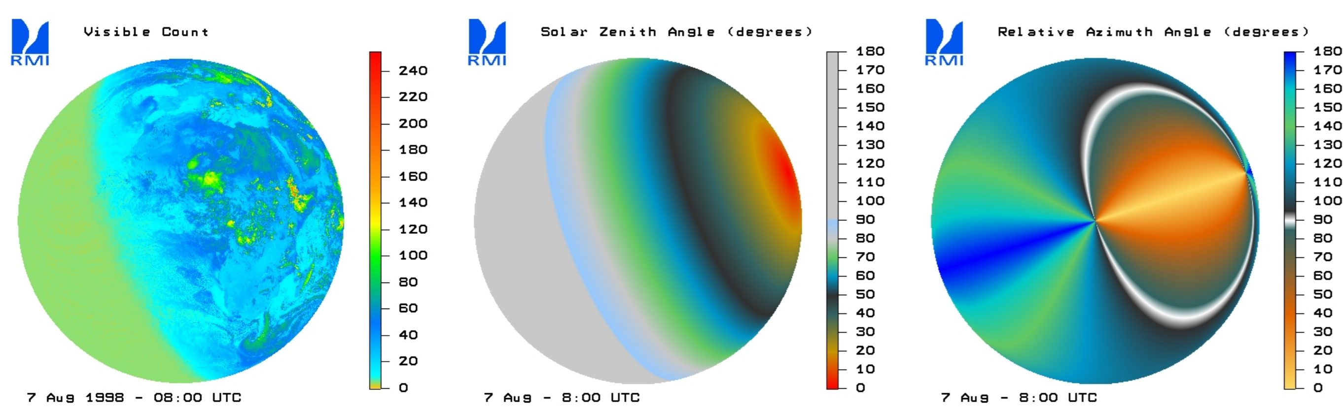
Figure 1: Left: Morning METEOSAT visible image. Mid: Corresponding solar zenith angles. Right: Corresponding relative azimuth angles.
