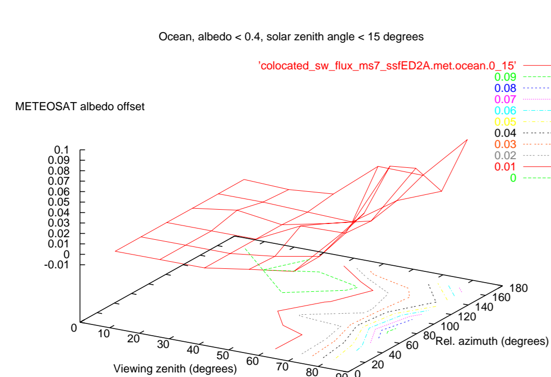
Figure 2: Offset of METEOSAT relative to mean CERES as a function of the viewing zenith and relative azimuth angle. Surface scene type: ocean. Solar zenith angles are between 0 and 15 degrees.
