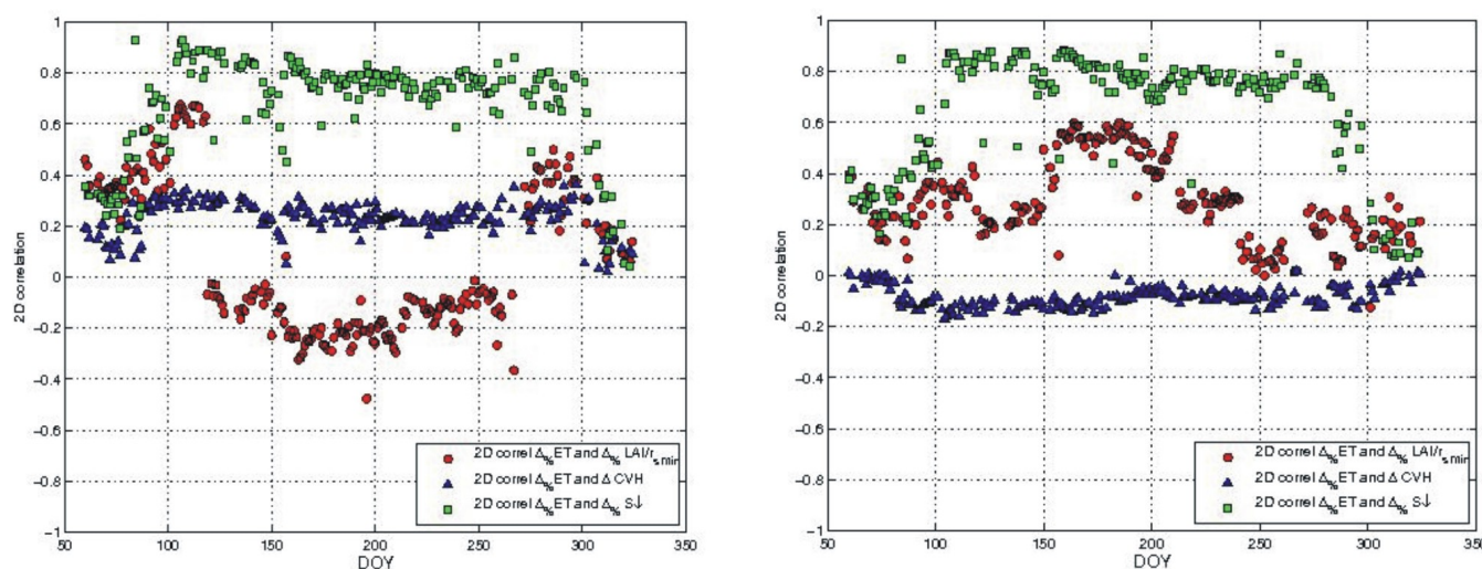
Fig. 8. Spatial (2-D) correlation over Europe between the ET mean relative bias (based on the images between 09:00 to 12:00 UTC) and model differences: (1) \text{LAI}/r_{s \text{ min}} (red diamonds), (2) High vegetation percentage (CVH, blue triangles), and (3) S_{\downarrow} mean relative bias (DSSF, green squares). At left: comparison between LSA SAF MET and ECMWF. At right: comparison between LSA SAF MET and GLDAS.
