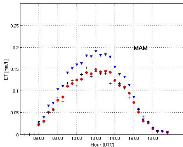
Fig. 2. Mean seasonal diurnal cycle of ET for the CarboEurope-IP Vielsalm station for March to May (MAM) 2007. Observation (+), pixel (v) and “tile” (o) estimate from LSA-SAF MET.
