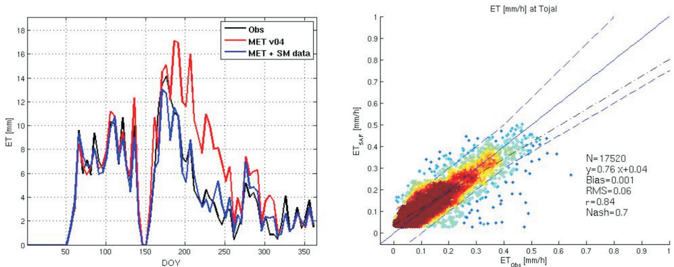
Fig. 9. Left: time series of the 5-days cumulated ET measured (black) and modelled (red) for the CarboEurope-IP Tojal station (Portugal) for the period from March to November 2007 as provided by LSA SAF MET. Modelled ET using soil moisture measured at the station (blue) has been superimposed. Right (as in Fig. 3) but modelled ET computed with soil moisture measured at the station compared to 30 min mean observed ET.
