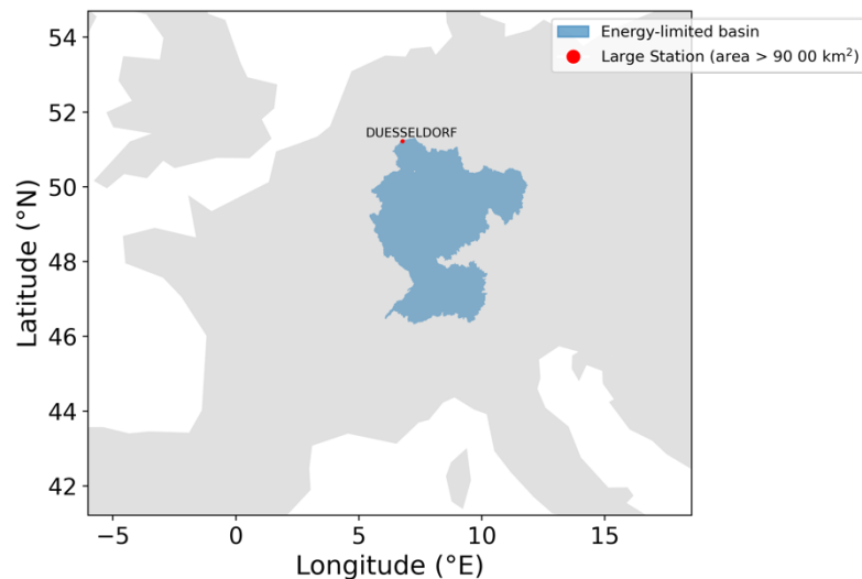
Figure 7: Location of the GRDC station Düsseldorf (red dot) and its associated river basin (blue polygon) derived from GRDC shapefiles (area of 147680 km 2 ). The basin, part of the Rhine River system, is classified as large (area > 90 000 km 2 ) and energy-limited ( AI \leq 1 ).
