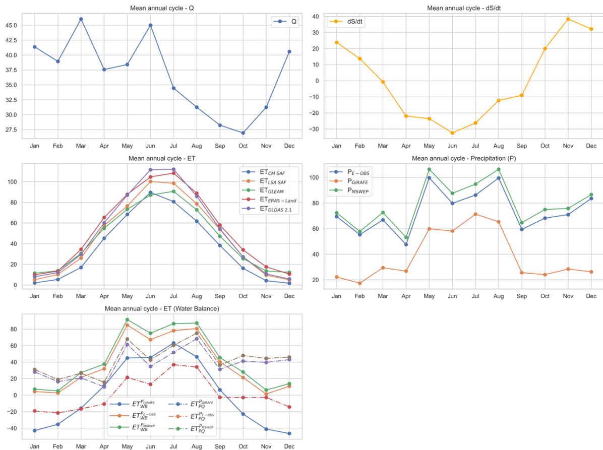
Figure 21: Mean annual cycles of hydrological variables over the Düsseldorf basin for the period 2004–2020. The top left panel shows the monthly climatology of river discharge (Q), while the top right panel displays the average monthly change in water
