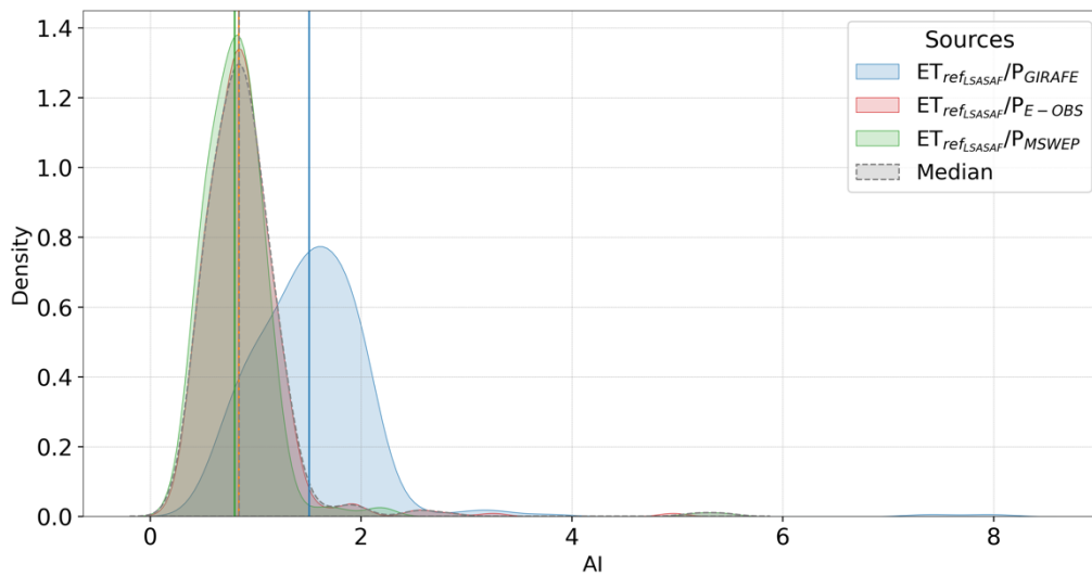
Figure 6: Probability density functions (PDFs) of the aridity index (AI), computed as the ratio of reference evapotranspiration from LSA SAF ( ET_{refLSA\ SAF} ) to precipitation (P), for all selected basins over the period 2004–2020. The analysis is based on three regridded ( 0.25^\circ ) precipitation datasets: GIRAFE (blue), E-OBS (red), and MSWEP (green). The grey-shaded area represents the distribution of median AI values derived from the three individual datasets. Vertical solid lines indicate the median AI for each dataset.
