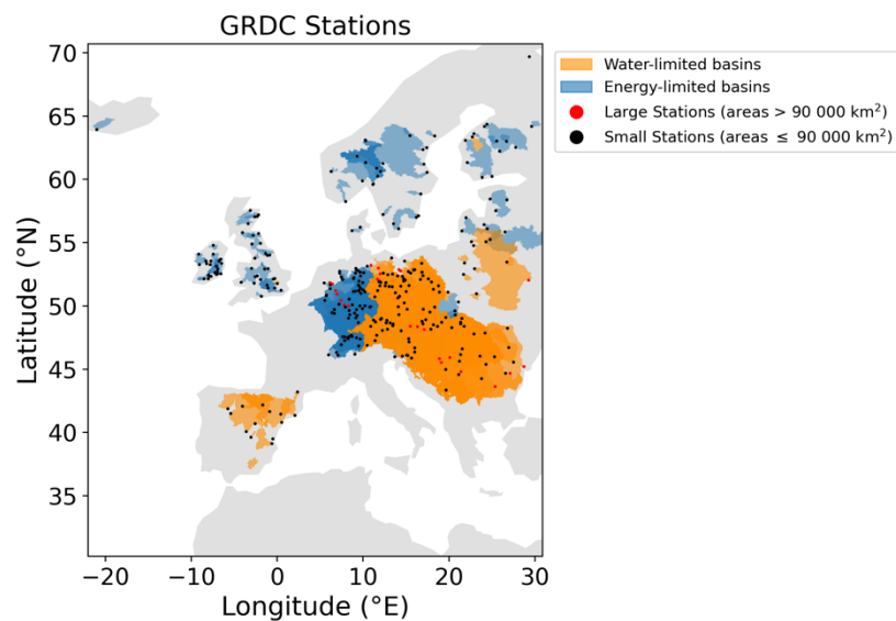
Figure 2: Spatial distribution of the 332 river discharge stations selected from the Global Runoff Data Centre (GRDC) across Europe. Each dot represents a station, with red indicating large basins (area > 90\,000 \text{ km}^2 ) and black indicating small basins (area \leq 90\,000 \text{ km}^2 ). The associated basin shapes are also shown, colored according to their aridity index (AI): blue for energy-limited basins ( \text{AI} \leq 1 ) and orange for water-limited basins ( \text{AI} > 1 ).
