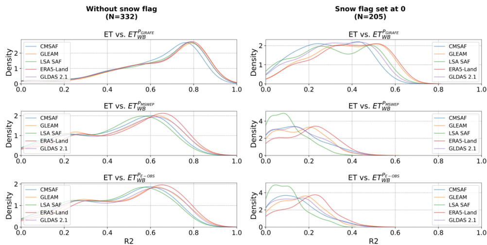
Figure 10: Probability density functions (PDFs) of R^2 values between independent evapotranspiration (ET) products (CM SAF, GLEAM, LSA SAF, ERA5-Land, GLDAS 2.1) and ET derived from the water balance-derived evapotranspiration estimates based using three different precipitation datasets: GIRAFE (top row, ET_{WB}^{GIRAFE} ), MSWEP (middle row, ET_{WB}^{MSWEP} ), and E-OBS (bottom row, ET_{WB}^{E-OBS} ). Left panels show results without applying a snow flag, while right panels include only values where the GIRAFE snow flag is set to 0. Each color represents one ET product, with N the number of basins considered.
