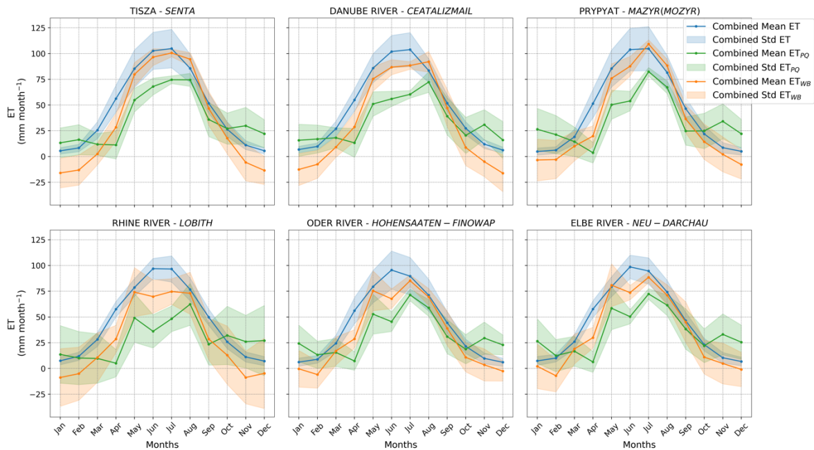
Figure 12: Monthly mean annual cycle (MMAC) of evapotranspiration ( \text{ET} ; \text{mm month}^{-1} ) estimated from different approaches for the six largest river basins from our database. Each panel represents a different basin, illustrating the average (solid line) and the standard deviation (shaded area) of the evapotranspiration MMAC. The estimates are derived from independent datasets (in blue) and from the water balance equation using different precipitation products, with (orange) and without (green) considering changes in water storage.
